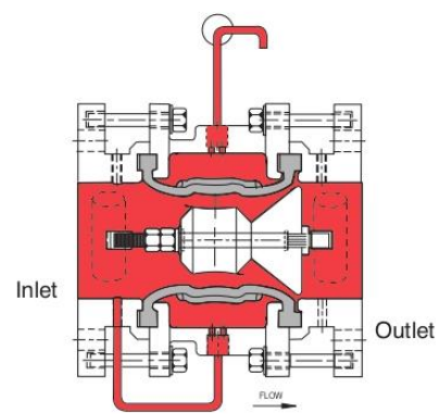
Modulating Action
