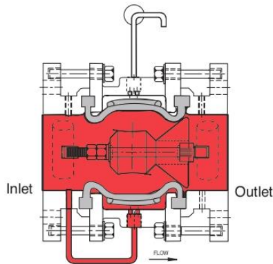
Full Open Operation
